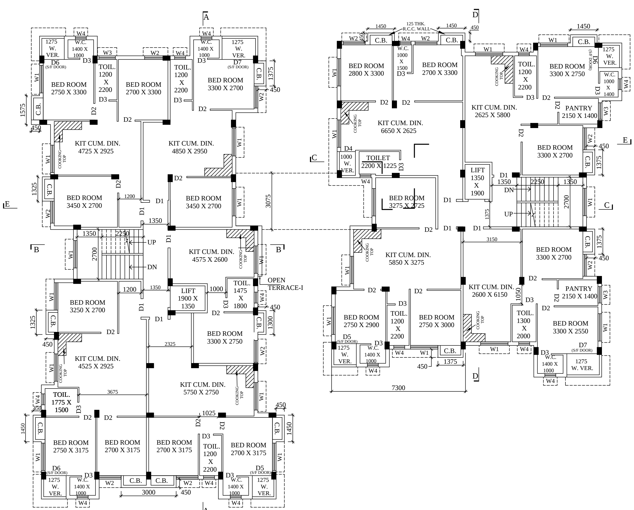
TYPICAL FLOOR PLAN (1ST TO 4TH) SCALE - 1:100
